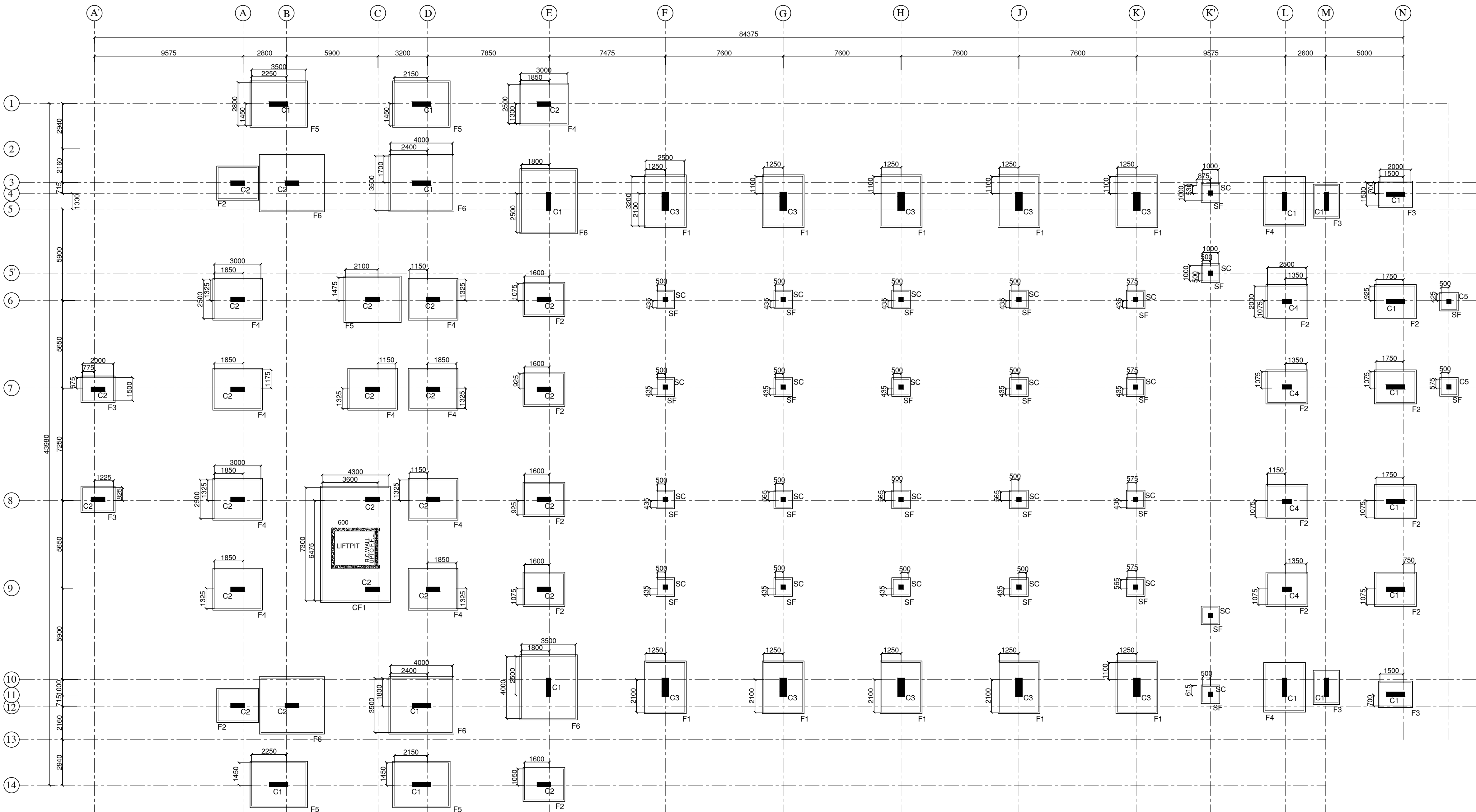
LAYOUT OF COLUMNS & FOOTINGS
