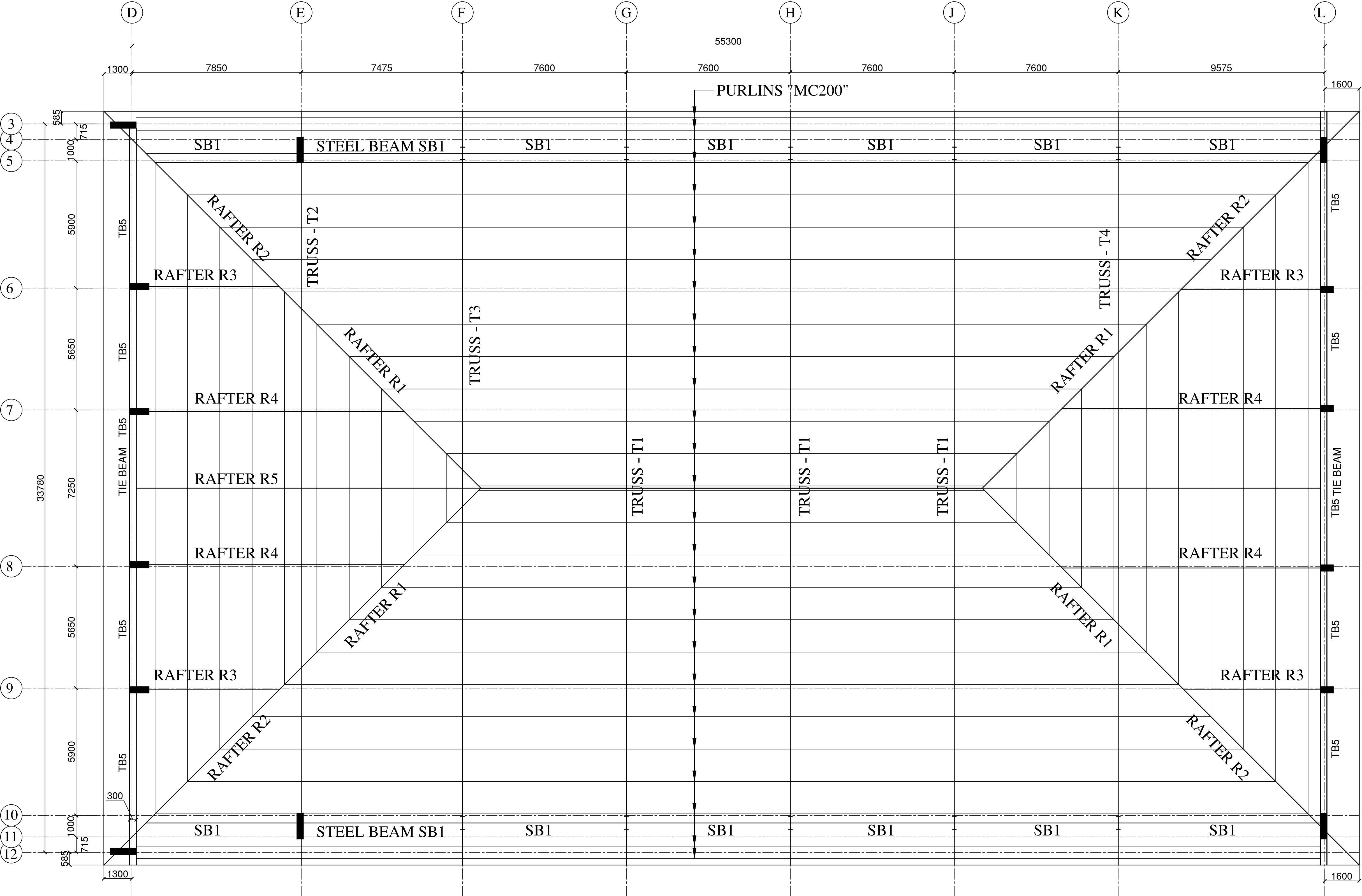
LAYOUT OF TRUSS AND PURLINS
