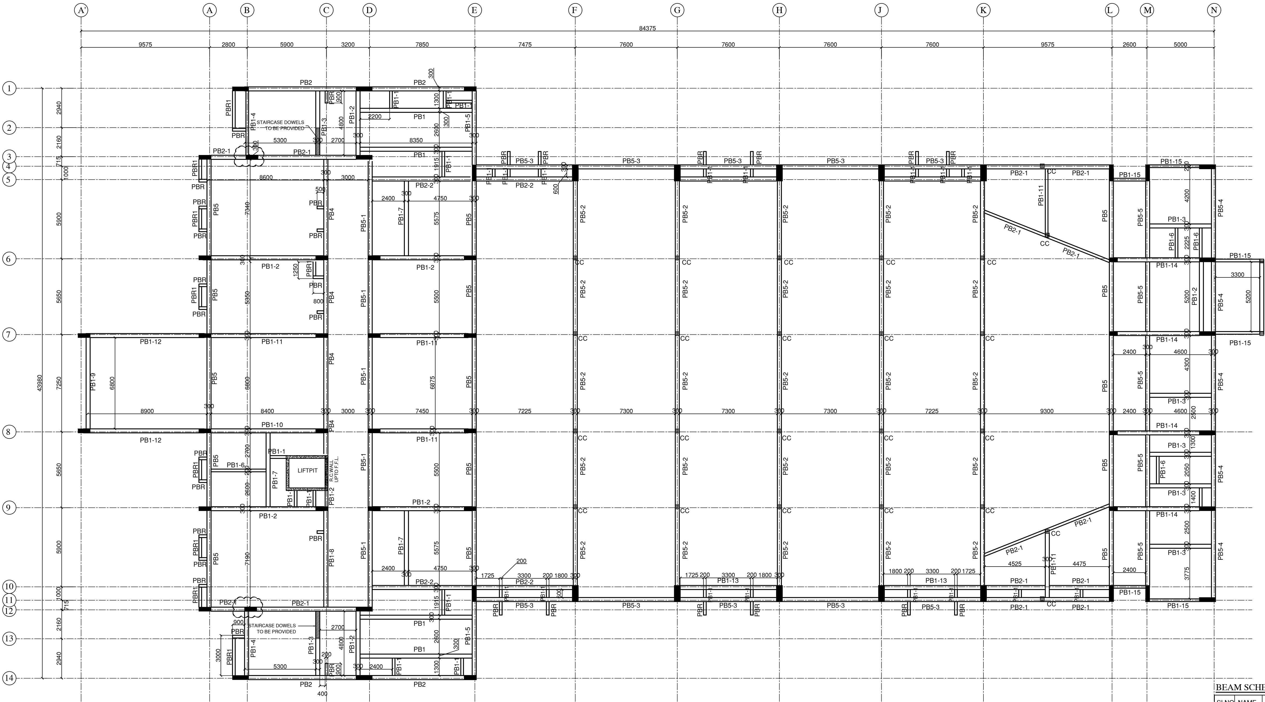
LAYOUT OF PLINTH BEAMS
